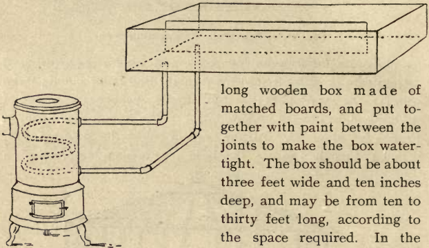
Fig. 39. Barnard's Propagating-tank.
